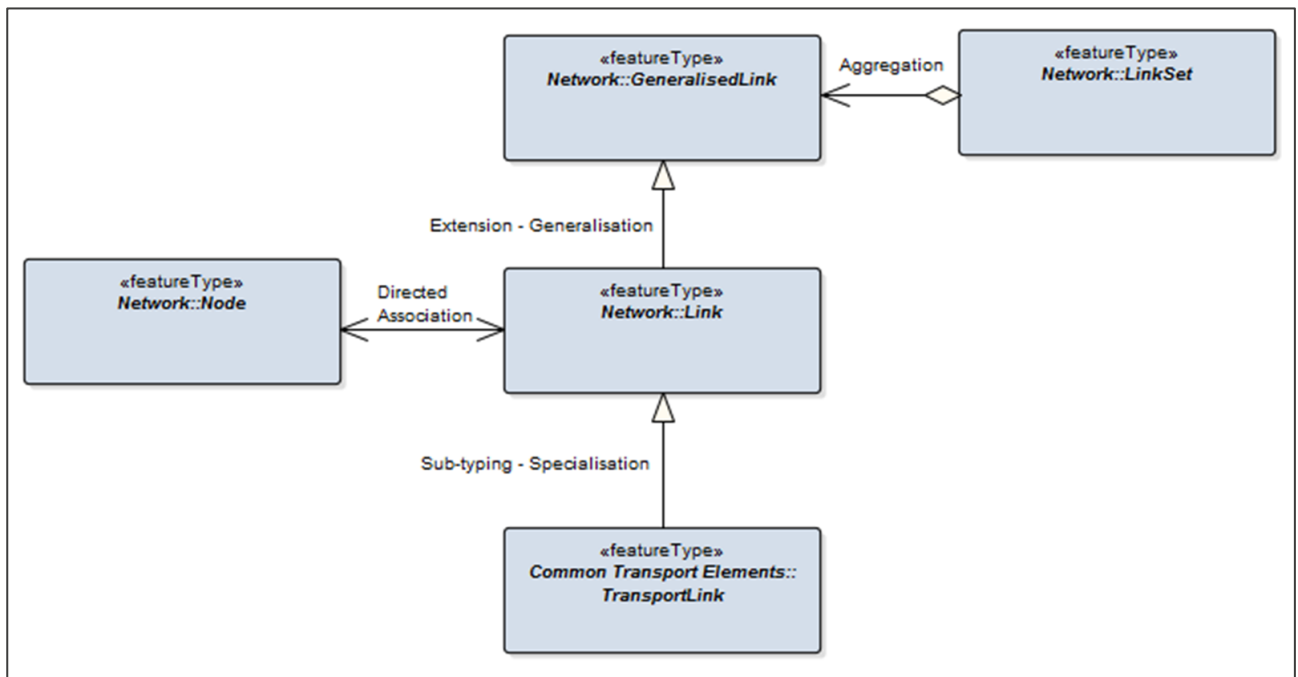
Figure 4. Relationships between feature types
