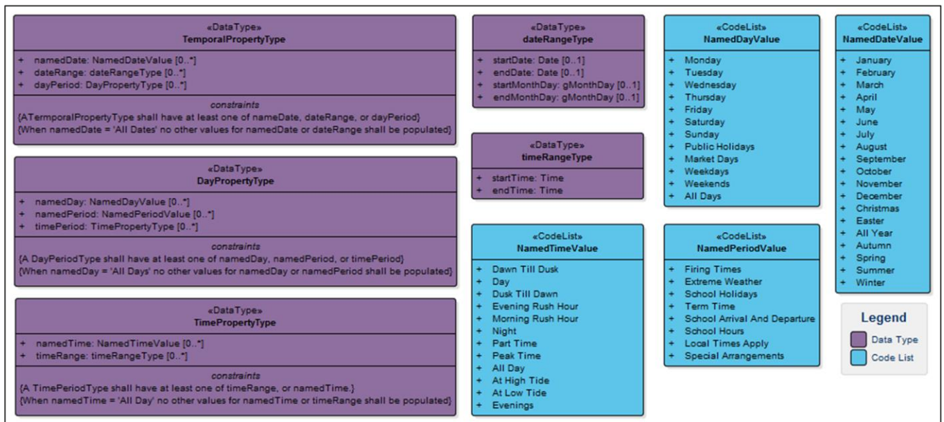
Figure 17.Components of the TemporalPropertyType
