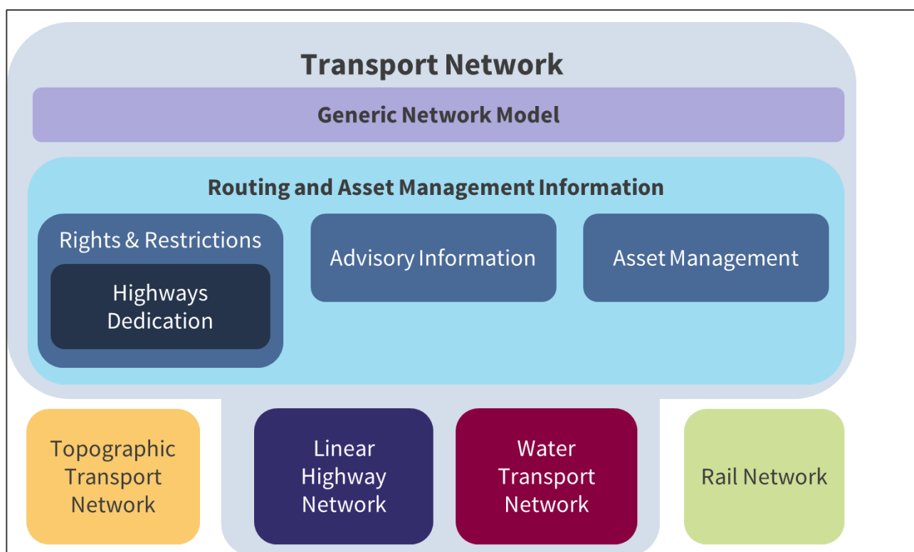
Figure I. The conceptual INSPIRE Transport Network Model
