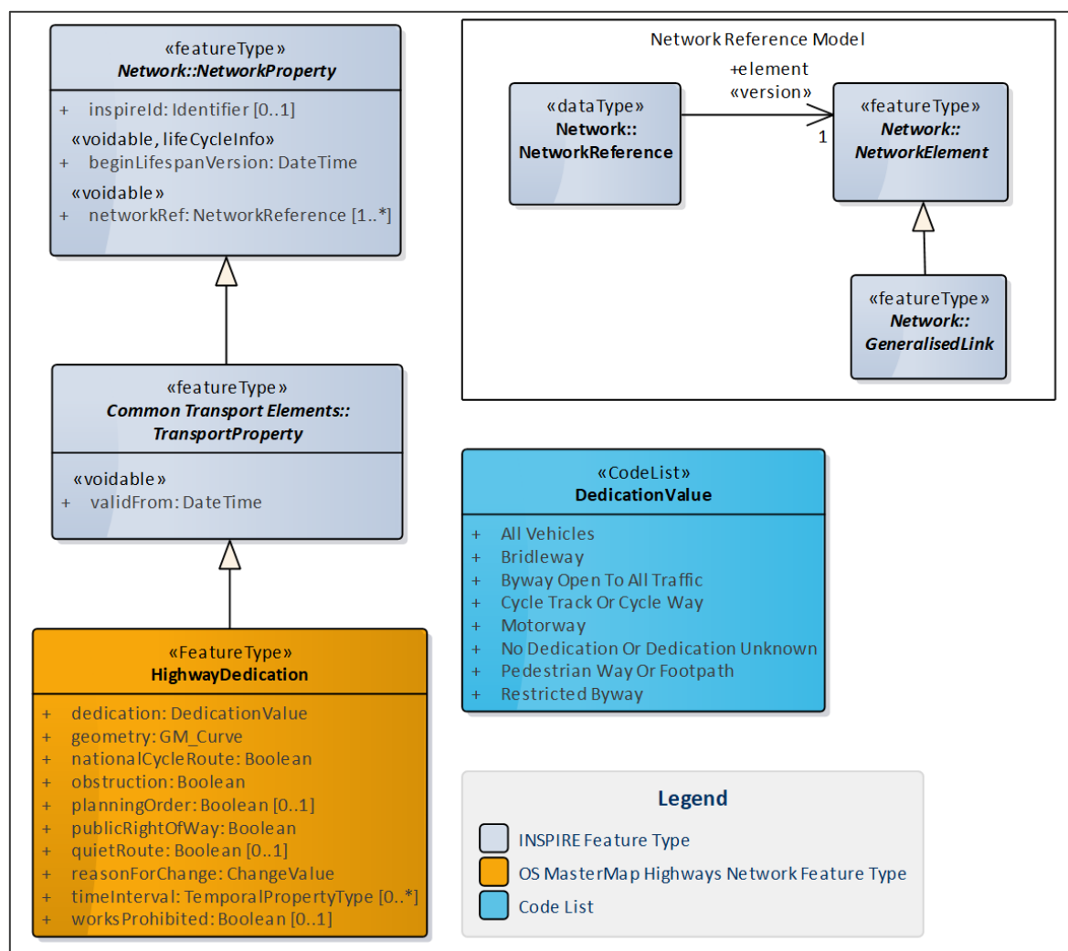
Figure 9. Context diagram: HighwayDedication
