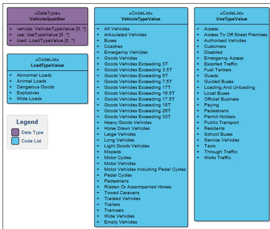
Figure 18.Components in the VehicleQualifier
