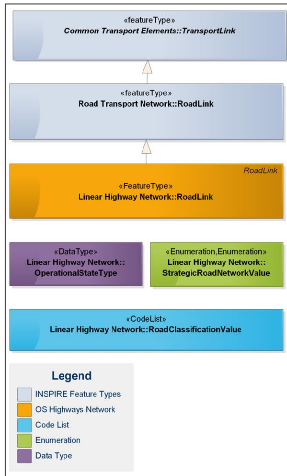
Figure 2. Colour conventions used in UML diagrams
