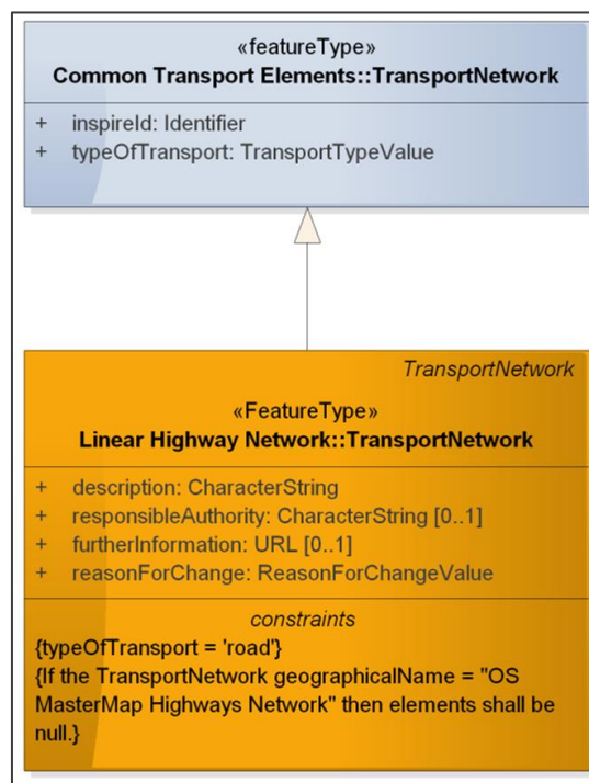
Figure 3. Representation of constraints in UML diagrams
