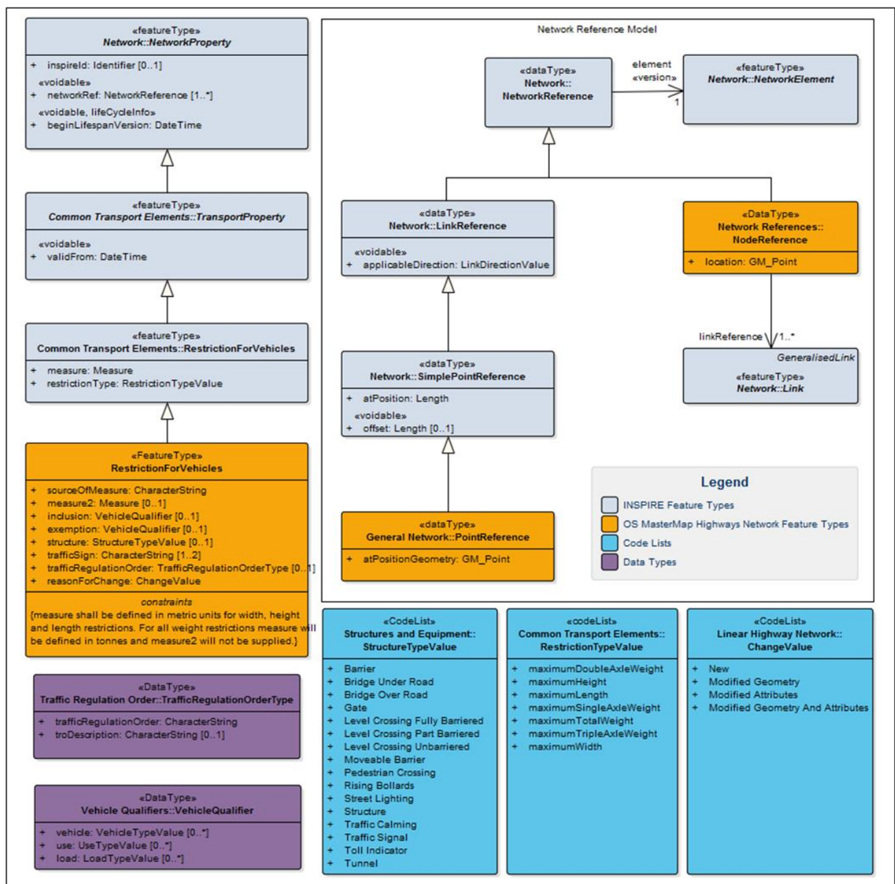
Figure 11. Context diagram: RestrictionForVehicles
