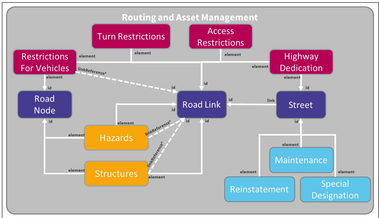
Figure 19.OS MasterMap Highways Network – Routing and Asset Management Information relational model
